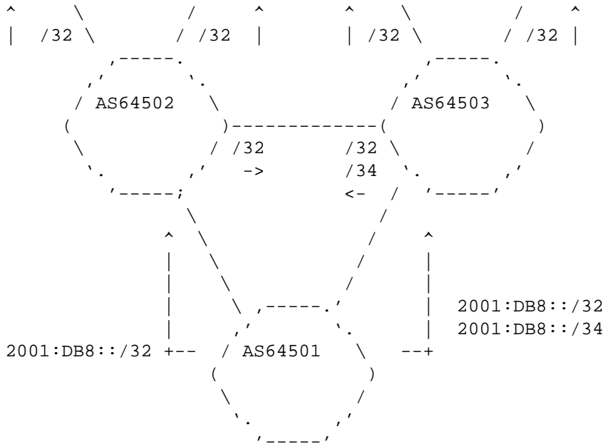
Figure 3: Remote triggered filtering
