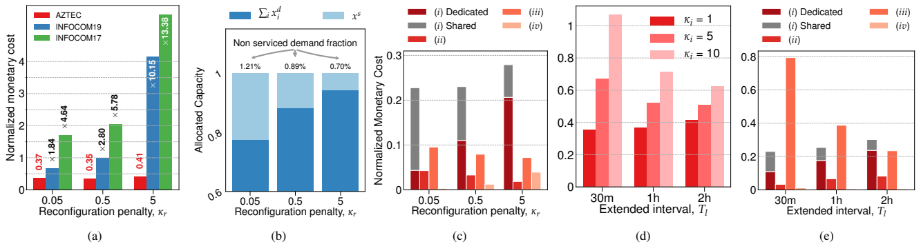
Fig. 5. Evaluation results. (a) Normalized monetary cost of AZTEC and two benchmarks versus the reconfiguration cost scaling factor \kappa_r . Numbers denote the exact cost for AZTEC, and the added cost factor for the benchmarks. (b) Total dedicated capacity \sum_{i \in \mathcal{S}} x_i^d(t) and shared capacity x^s(t) allocated by AZTEC versus \kappa_r . Numbers denote the fraction of re-orchestration opportunities with insufficient allocated resources. (c) Breakdown of the normalized monetary cost by penalty type. Tags refer to cost definitions in Section II-A, with overprovisioning cost (i) separated into contributions of the dedicated capacity, i.e. , the first term of (1), and of the shared capacity, i.e. , the second and third terms of (1). (d) Normalized monetary cost vs the duration of the extended re-orchestration interval T_l , for different scaling factors \kappa_i of the resource instantiation cost. (e) Breakdown of the normalized monetary cost by penalty type, for \kappa_i = 10 .
