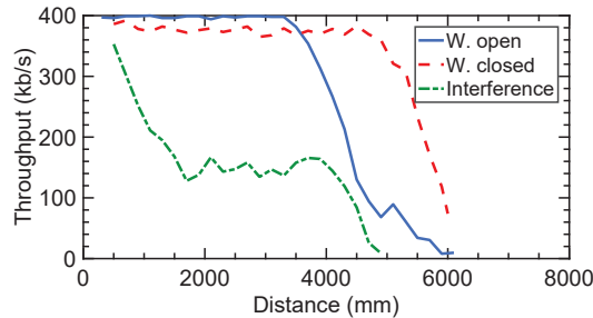
Fig. 7: UDP throughput as a function of the distance.
