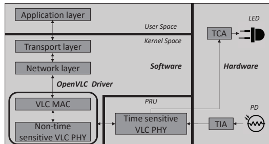
Fig. 2: The diagram of OpenVLC1.3.
