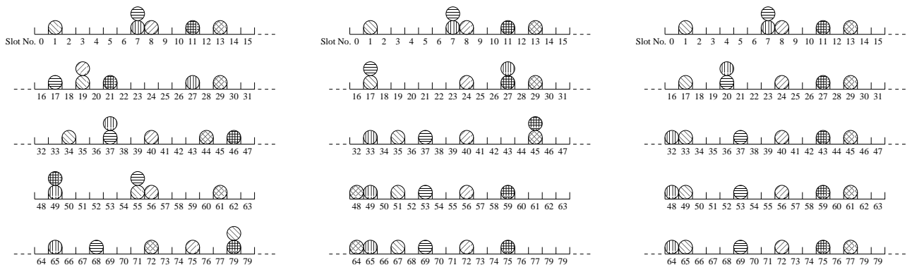
Fig. 1. An example of CSMA/CA (left), CSMA/ECA (center) and ZeroCollision (right) execution.
