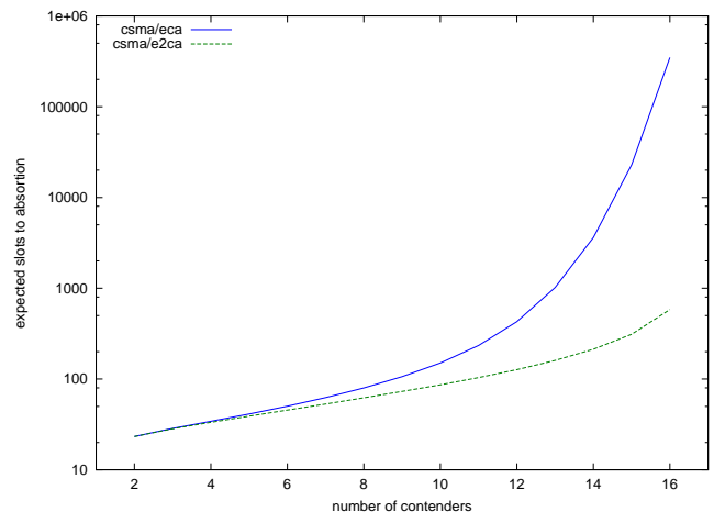
Fig. 4. Expected number of slots required to reach collision-free operation in CSMA/ECA and CSMA/E2CA for various numbers of contenders.
