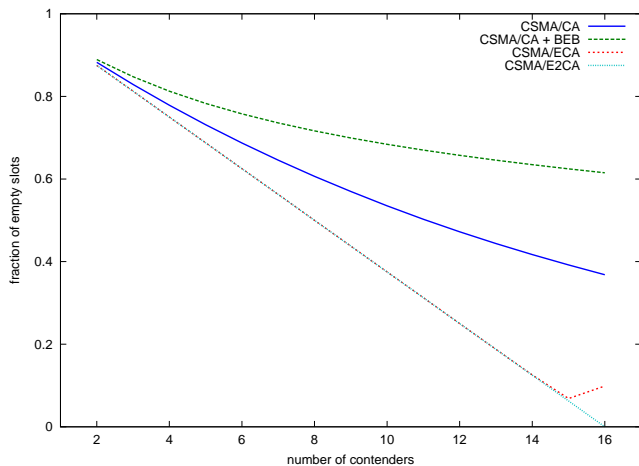
Fig. 5. Fraction of empty slots for each of the three protocols under comparison for different number of contenders.
