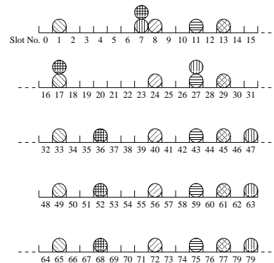
Fig. 3. A graphical example of the execution of CSMA/E2CA
