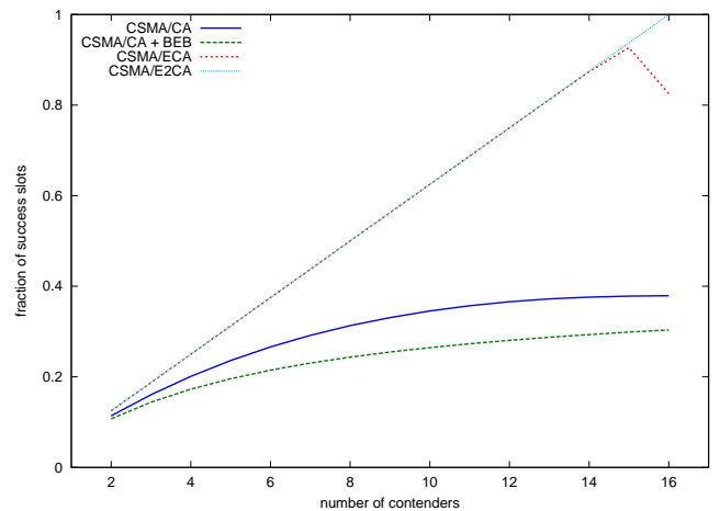
Fig. 7. Fraction of success slots for each of the three protocols under comparison for different number of contenders.
