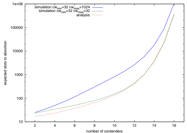
Fig. 2. Number of expected slots to reach collision-free operation in CSMA/ECA.
