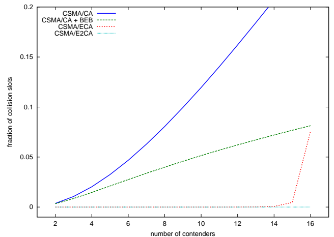
Fig. 6. Fraction of collision slots for each of the three protocols under comparison for different number of contenders.
