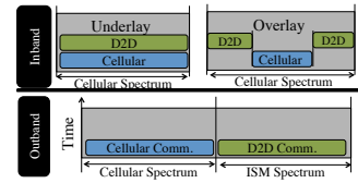
Figure 2: Schematic representation of overlay inband, underlay inband, and outband D2D.
