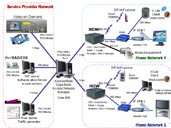
Figure 2: Testbed for the QoS trials
