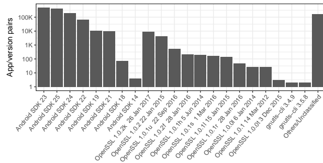
Figure 2: Rank of TLS libraries by unique app-version pairs (log10-scale). Most apps use OS-provided APIs with default settings.
