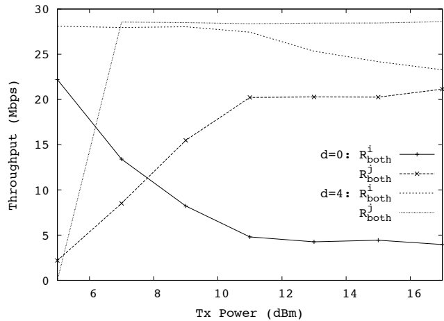
Fig. 17. Impact of channel separation and transmitted power on bandwidth share.
