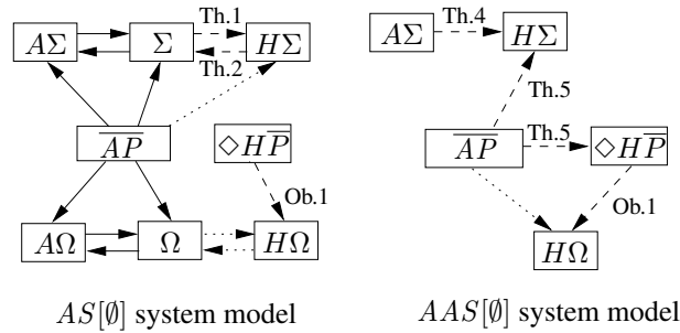
Figure 5: Relations between failure detector classes in the models AS[\emptyset] and AAS[\emptyset] . There is an arrow from class X to X' if X is stronger than X' . Solid arrows are relations shown by Bonnet and Raynal in [6]. Dotted arrows are trivial relations. Dashed arrows are relations shown here (the arrow label shows the theorem or observation where the relation is proven).
