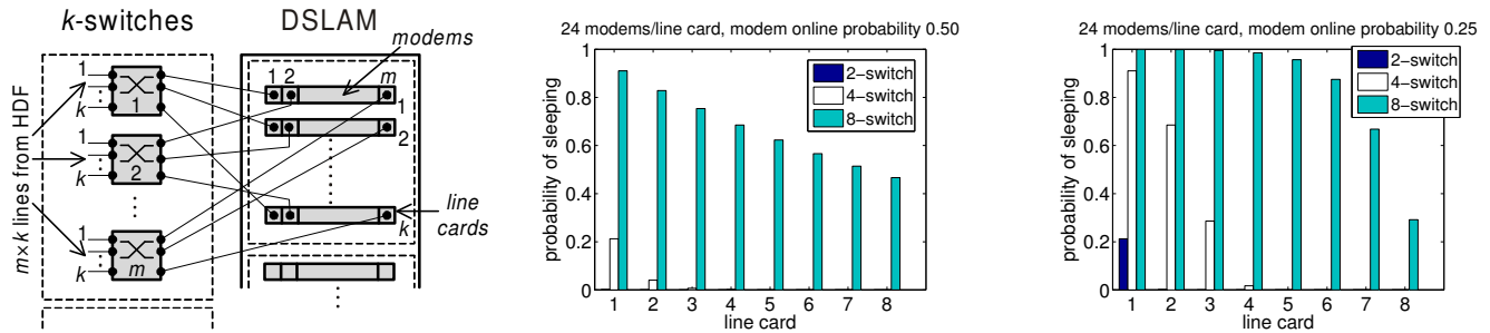
Figure 5: [left] k -switches and connection to DSLAM. [middle and right] Probability of line card 1, 2, \dots , k sleeping on a batch of k line cards connected through m k -switches. Each line card has m = 24 modems and each modem is active with probability p = 0.5 (middle) or p = 0.25 (right).
