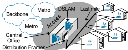
Figure 1: Illustration of a residential DSL broadband network. User gateways are connected to DSLAM ports via telephone lines in shared bundles up to few km long.
