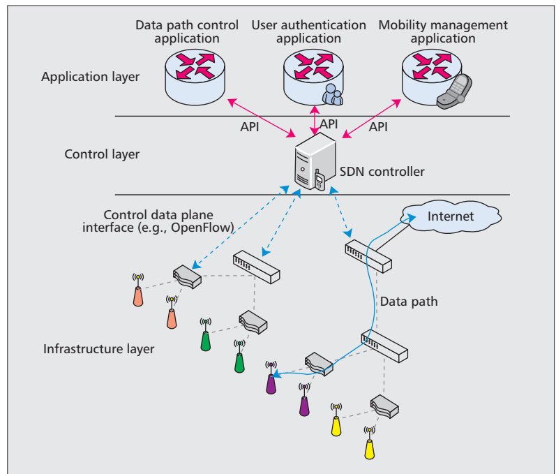
Figure 1. SDN reference architecture.
