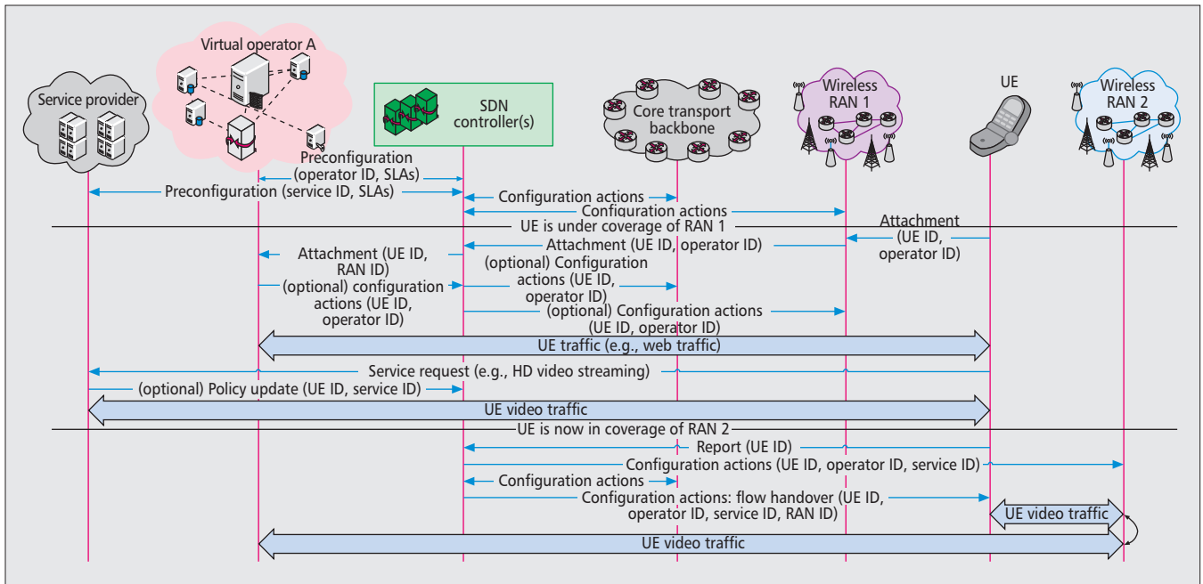
Figure 4. Case study: SDWN high-level interactions.
